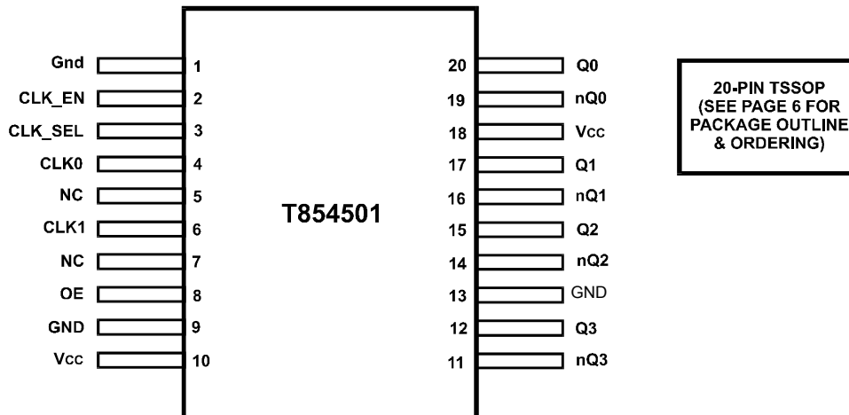
Figure 2. Pin Configuration
